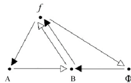
Figure 1. Rosen’s relational model of closure to efficient causation. White arrows represent relations of material causation; black arrows represent relations of efficient causation.
